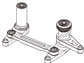
完成図 Picture of assembled product.
