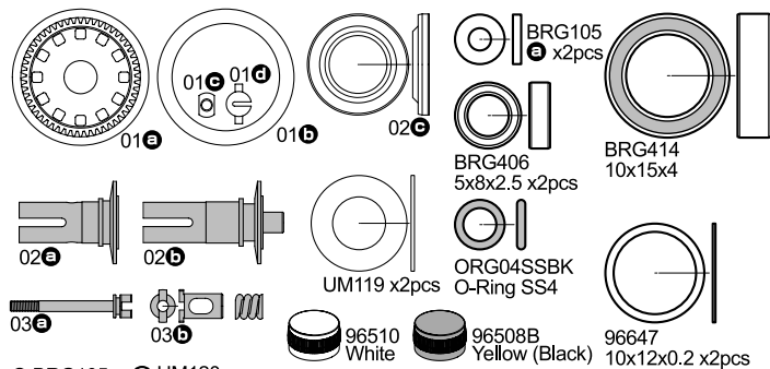
BRG105 a x2pcs BRG406 5x8x2.5 x2pcs BRG414 10x15x4 UM119 x2pcs ORG04SSBK O-Ring SS4 96510 White 96508B Yellow (Black) 96647 10x12x0.2 x2pcs Ball Diff (for Belt Drive / OPTIMA) ボールデフ (ベルトドライブ用/オブティマ)
