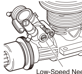
Low-Speed Needle Screw
